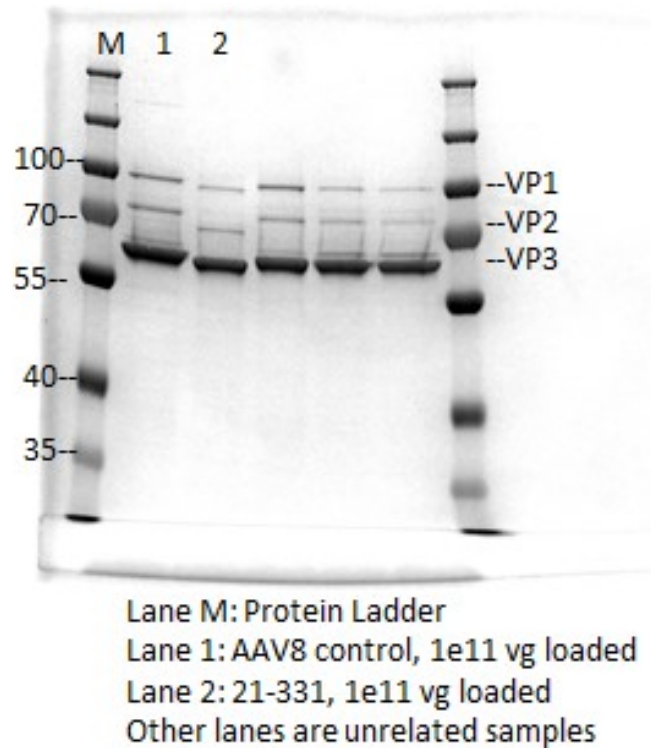
Fig. 1. SDS-PAGE and InstantBlue Staining of purified AAV2-CMV-GFP (Lot: 21-331).
