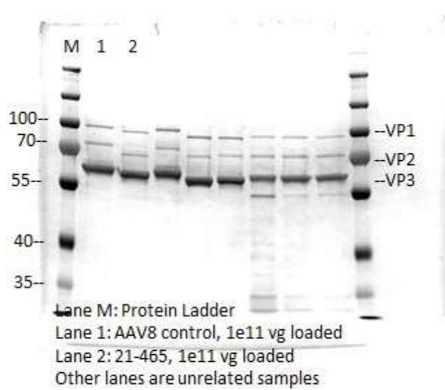
Fig. 1. SDS-PAGE and InstantBlue Staining of purified AAV2-CMV-GFP (Lot: 21-465).
