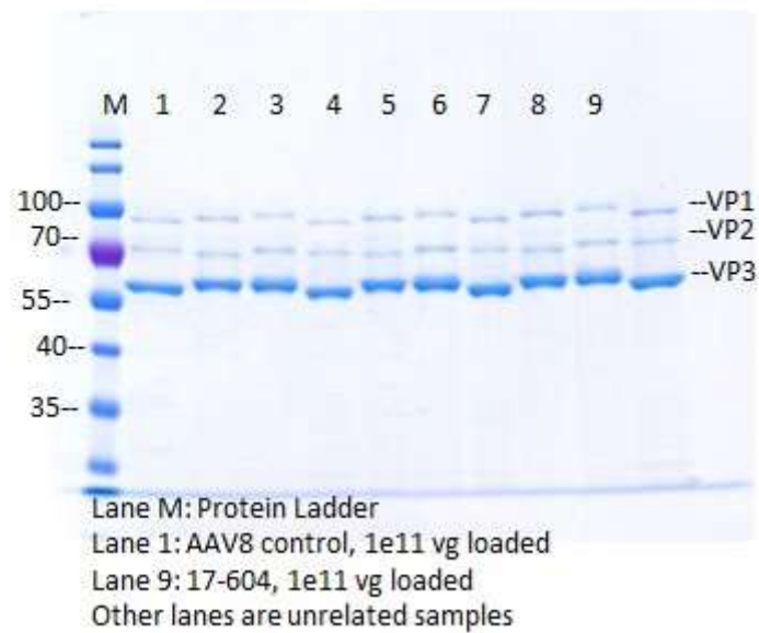
Fig. 1. SDS-PAGE and InstantBlue Staining of purified AAV5-CMV-GFP (Lot: 17-604).
