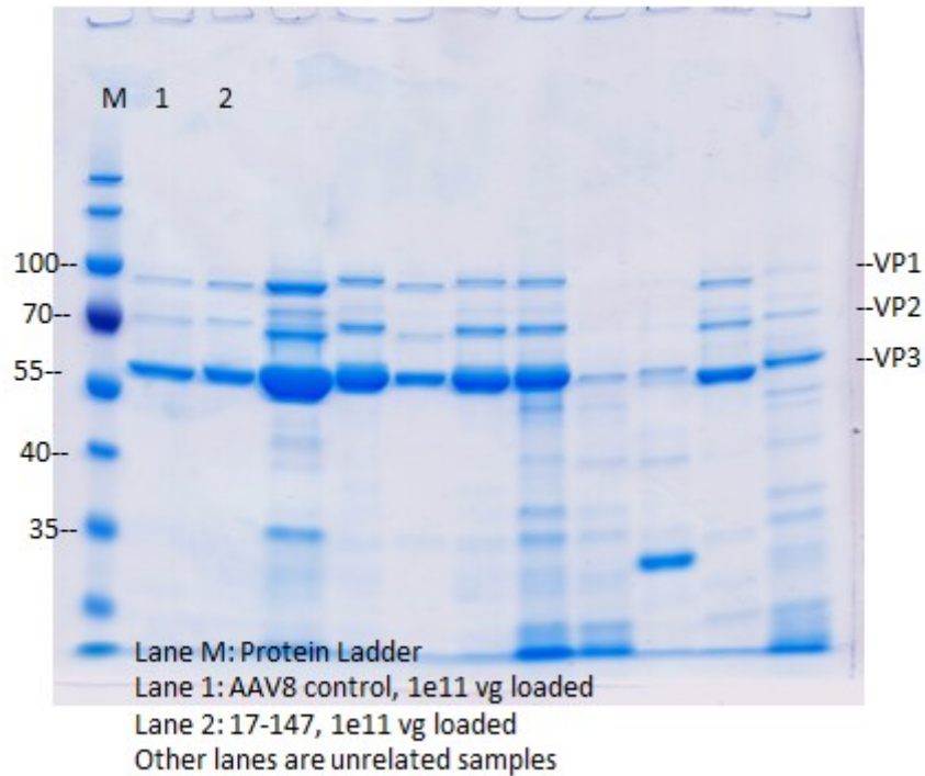
Fig. 1. SDS-PAGE and InstantBlue Staining of purified AAV6-CMV-GFP (Lot: 17-147).
