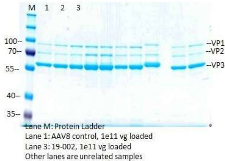
Fig. 1. SDS-PAGE and InstantBlue Staining of purified AAV9-CMV-Luciferase (Lot: 19-002).
